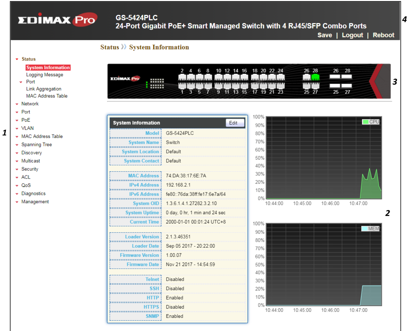
Figure 14 - User Interface
